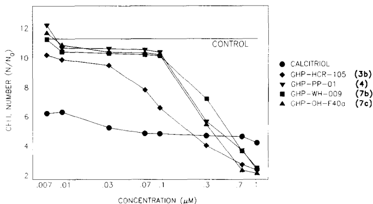
Figure 1. Dose response effects of dimers on keratinocyte proliferation (96 h).
