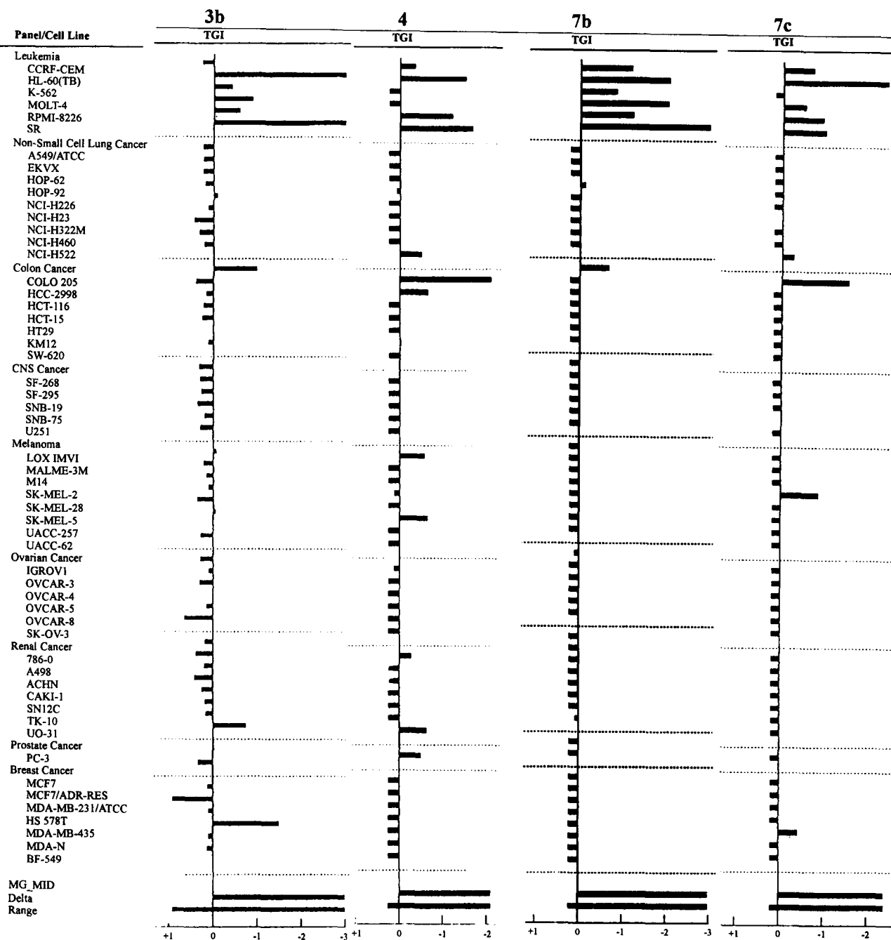
Figure 2. NCI 60 cell line assay.
